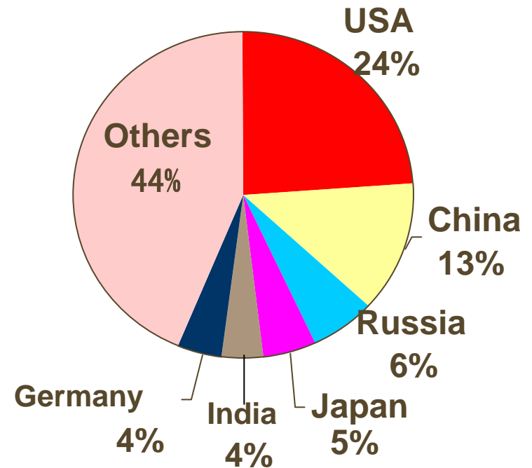
Global CO 2 emissions in 1999
